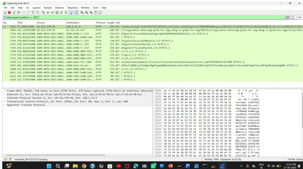
Figure 3: Applying Display Filter for HTTP Protocol
